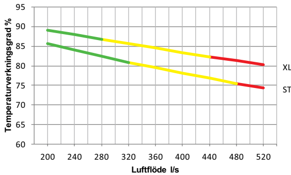
LTS Victum 4 200 - 520 l/s
