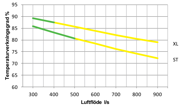
LTS Victum 5 300 - 900 l/s
