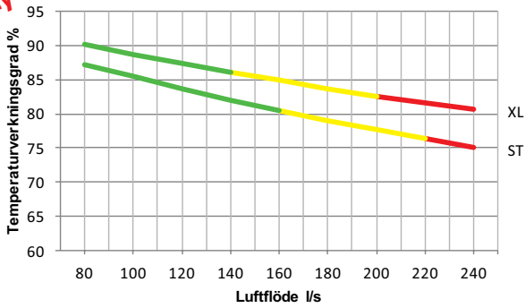
LTS Victum 2 80 - 240 l/s
