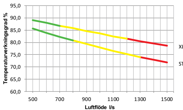
LTS Victum 6 500 - 1500 l/s
