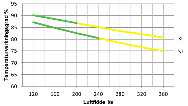
LTS Victum 3 120 - 360 l/s
